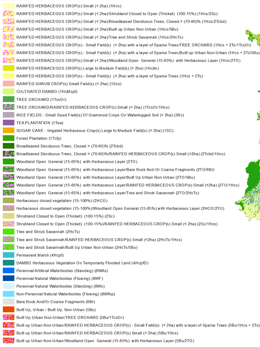
Figure 7.3.1 Malawi Land Cover 2010—FAO LCCS Full Resolution
